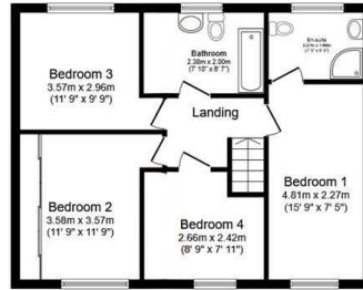
First Floor Floor area 55.3 sq.m. (595 sq.ft.)
