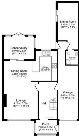
Ground Floor Floor area 87.2 sq.m. (938 sq.ft.)
